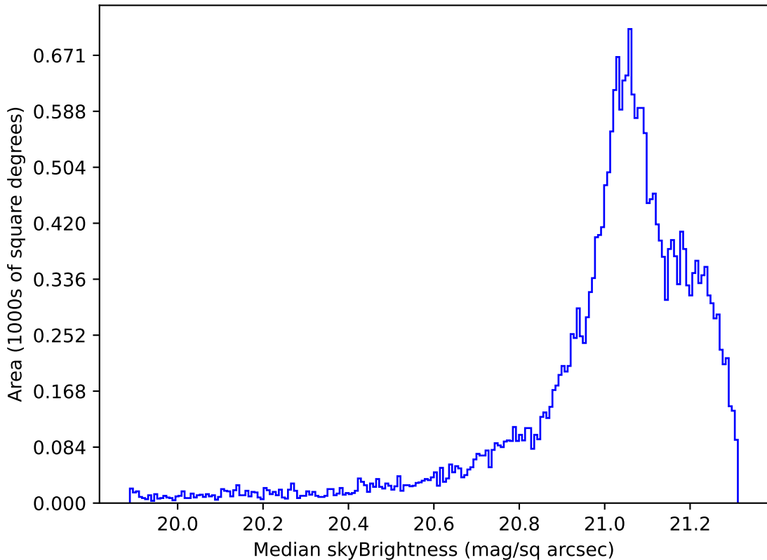
too_elab_r64_d2_griz_v3.4_10yrs Yr 1 r band: Median skyBrightness
