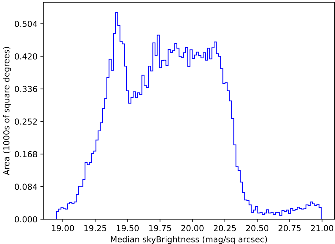
too_elab_r64_d2_griz_v3.4_10yrs Yr 1 all bands: Median skyBrightness
