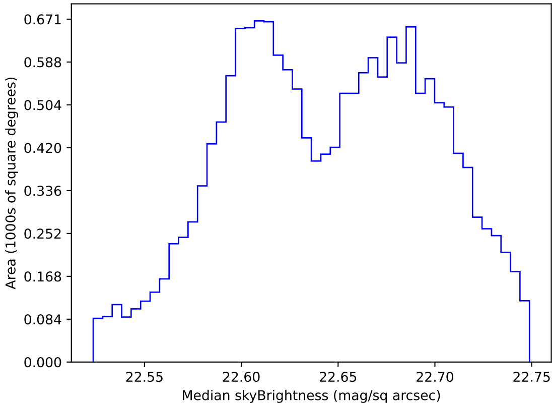
too_elab_r64_d2_griz_v3.4_10yrs WFD u band: Median skyBrightness
