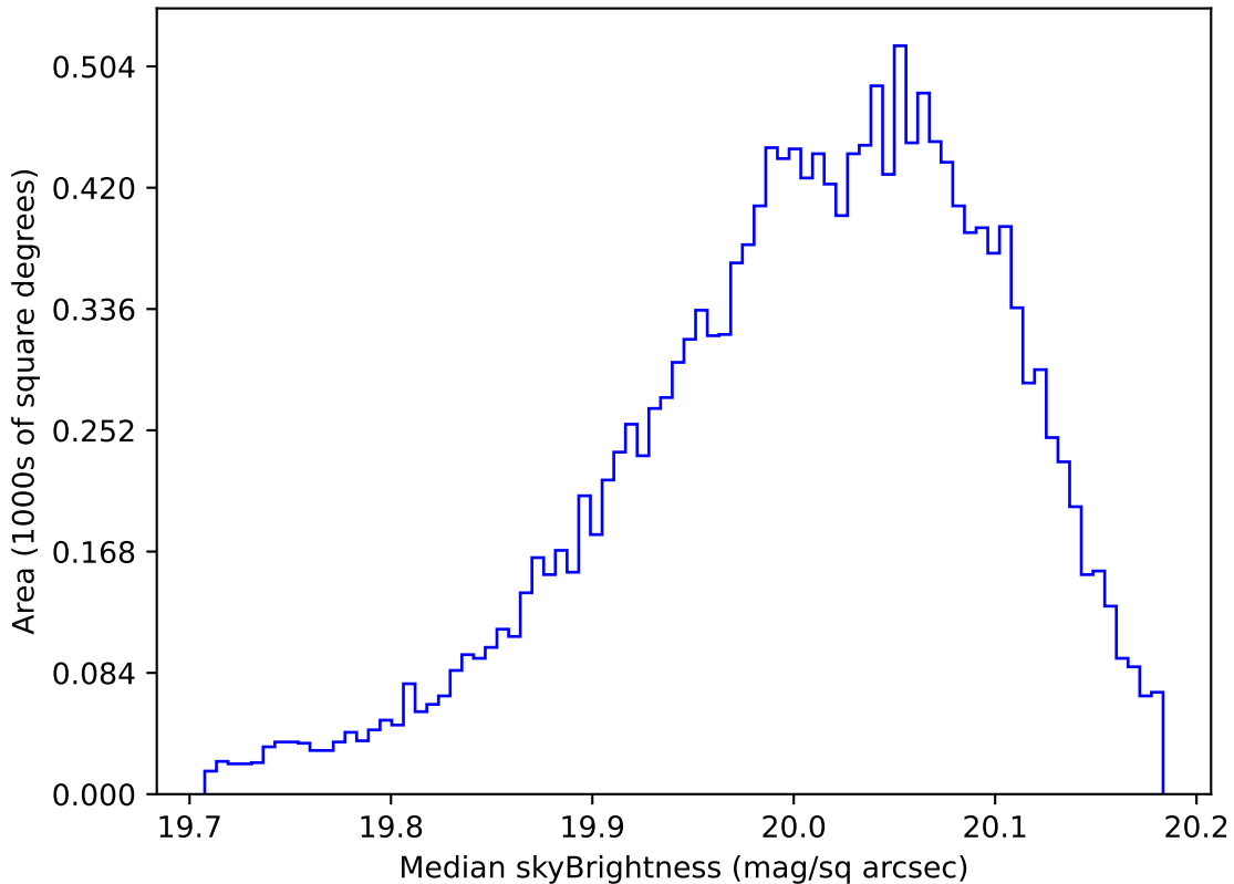
too_elab_r64_d2_griz_v3.4_10yrs WFD i band: Median skyBrightness
