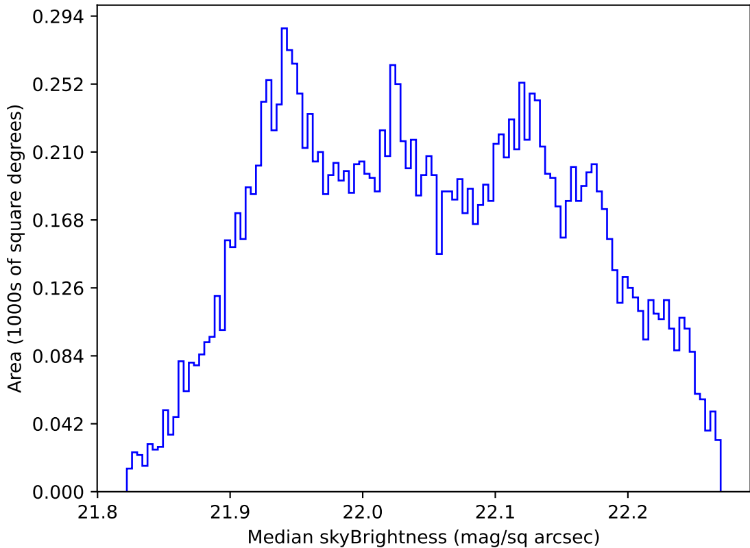
too_elab_r64_d2_griz_v3.4_10yrs WFD g band: Median skyBrightness
