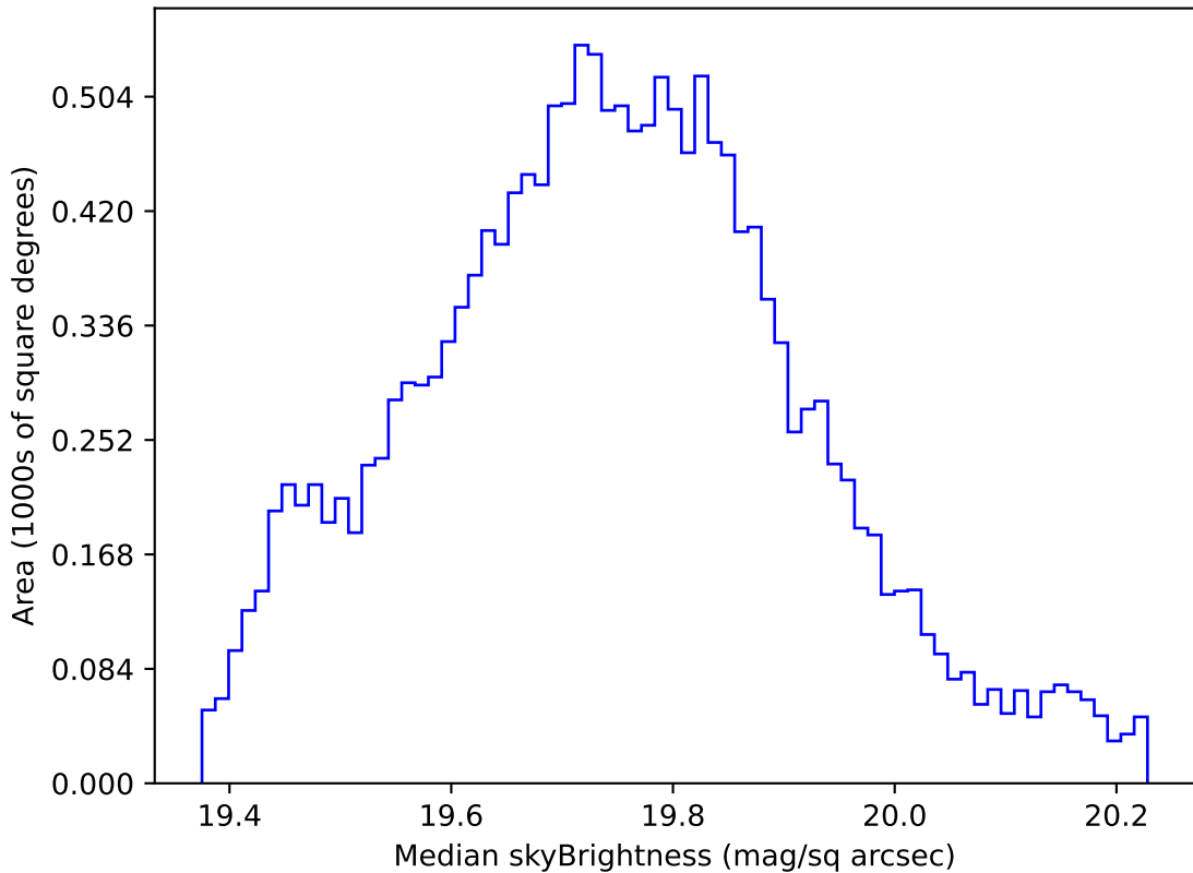
too_elab_r64_d2_griz_v3.4_10yrs WFD all bands: Median skyBrightness
