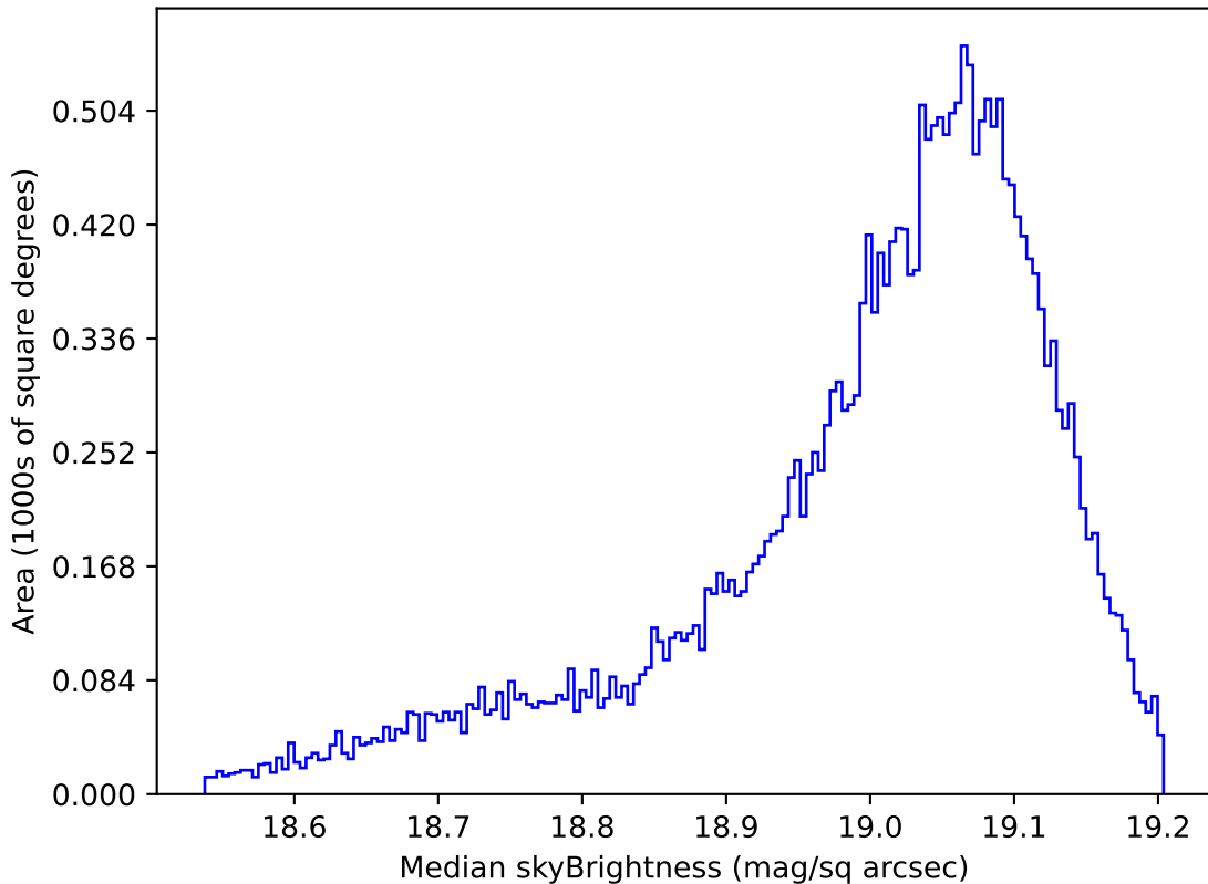
too_elab_r64_d2_griz_v3.4_10yrs All sky z band: Median skyBrightness
