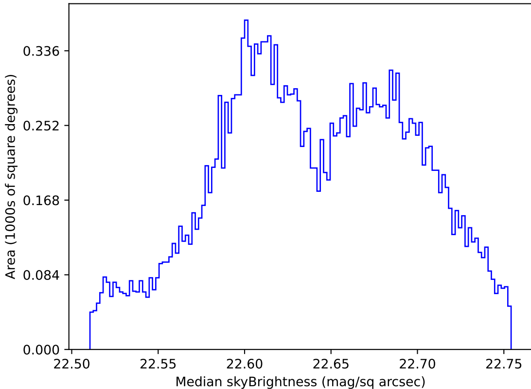
too_elab_r64_d2_griz_v3.4_10yrs All sky u band: Median skyBrightness
