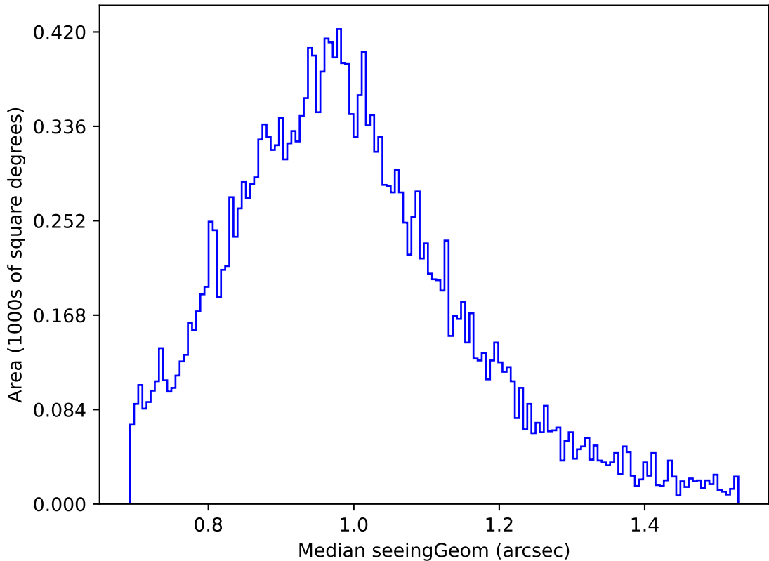
too_elab_r64_d2_griz_v3.4_10yrs Yr 1 u band: Median seeingGeom
