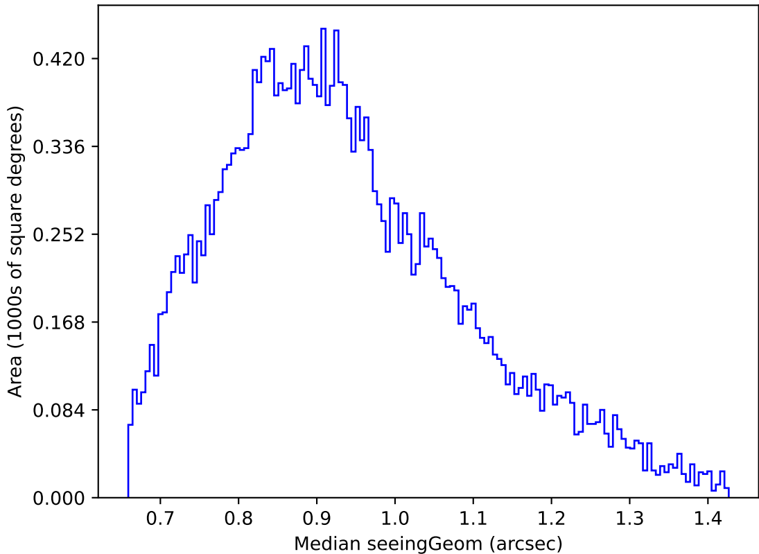
too_elab_r64_d2_griz_v3.4_10yrs Yr 1 g band: Median seeingGeom
