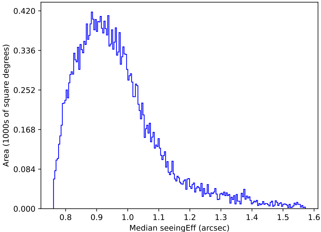
too_elab_r64_d2_griz_v3.4_10yrs Yr 1 z band: Median seeingEff
