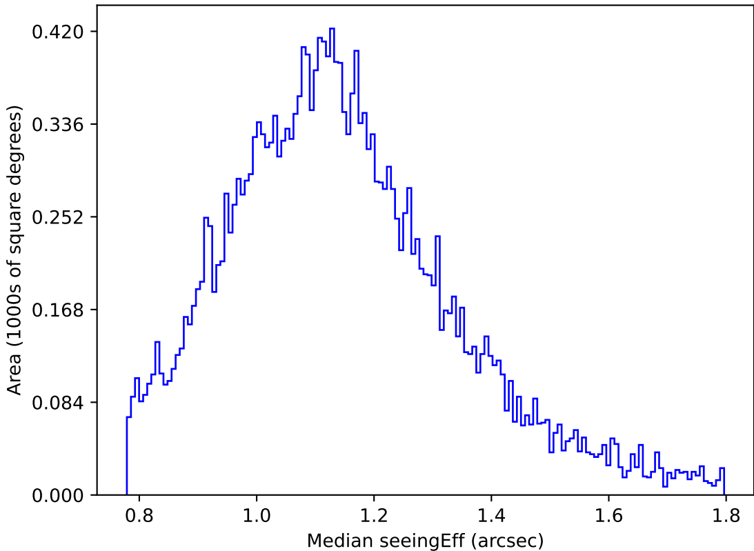
too_elab_r64_d2_griz_v3.4_10yrs Yr 1 u band: Median seeingEff
