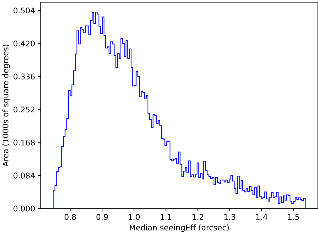
too_elab_r64_d2_griz_v3.4_10yrs Yr 1 r band: Median seeingEff
