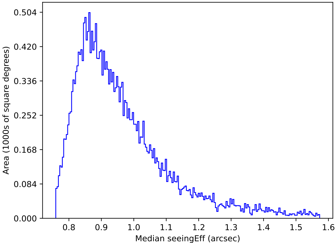
too_elab_r64_d2_griz_v3.4_10yrs Yr 1 i band: Median seeingEff
