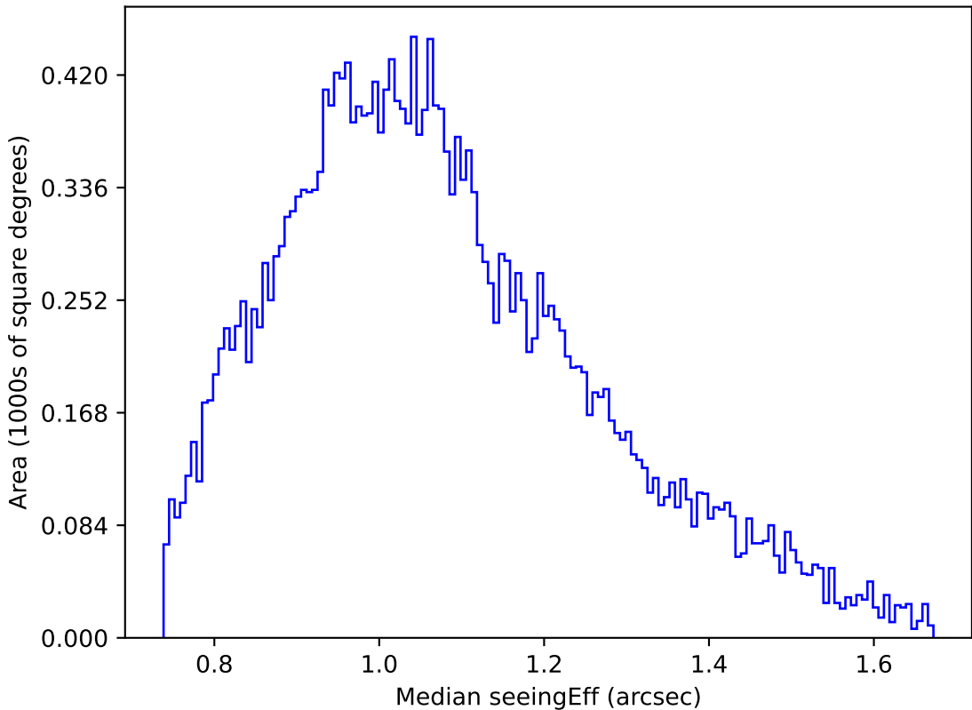
too_elab_r64_d2_griz_v3.4_10yrs Yr 1 g band: Median seeingEff
