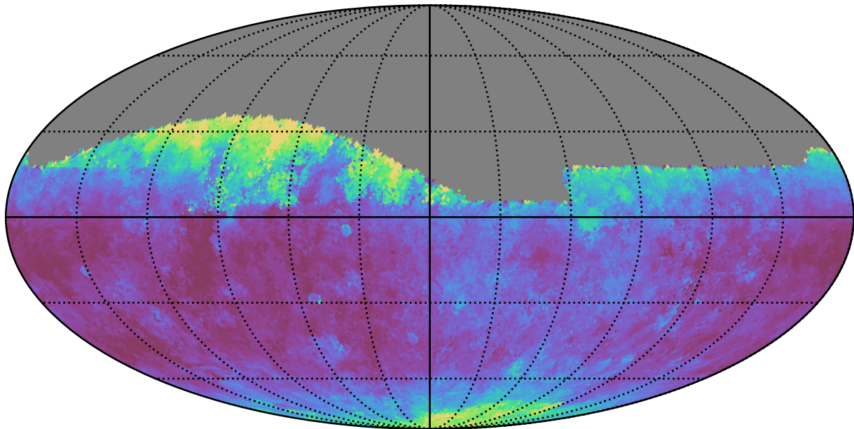
too_elab_r64_d2_griz_v3.4_10yrs Yr 1 all bands: Median seeingEff
