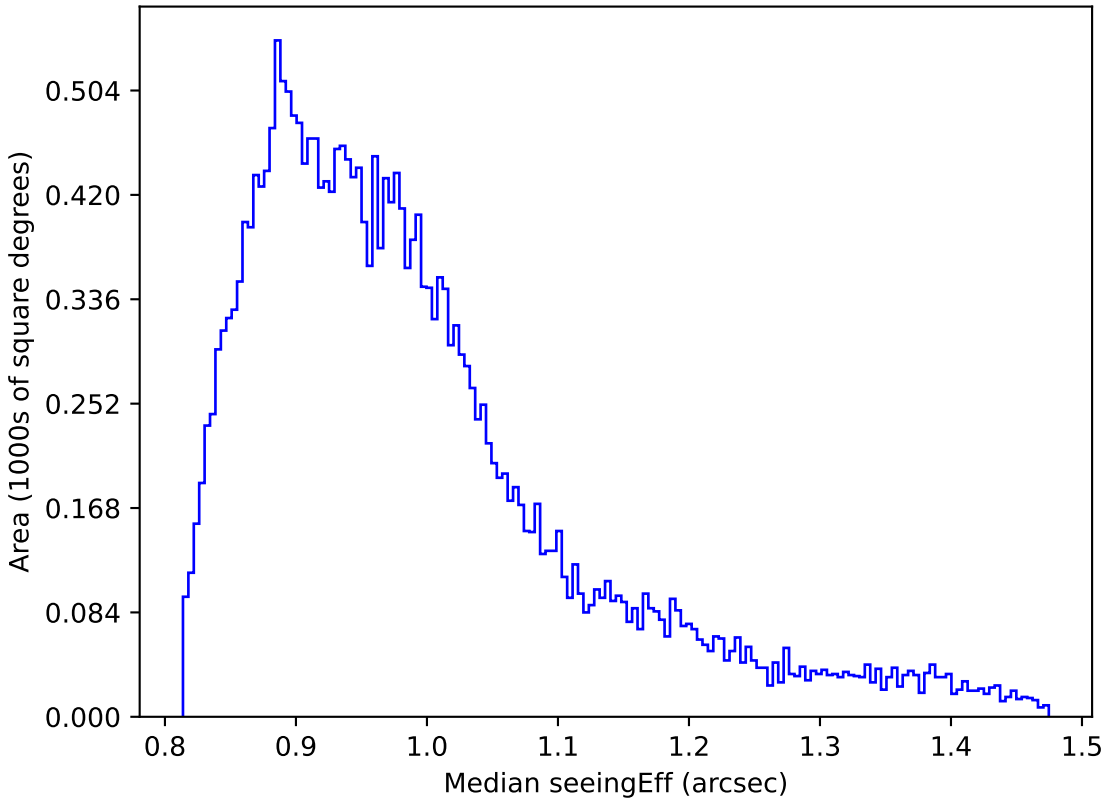
too_elab_r64_d2_griz_v3.4_10yrs Yr 1 all bands: Median seeingEff
