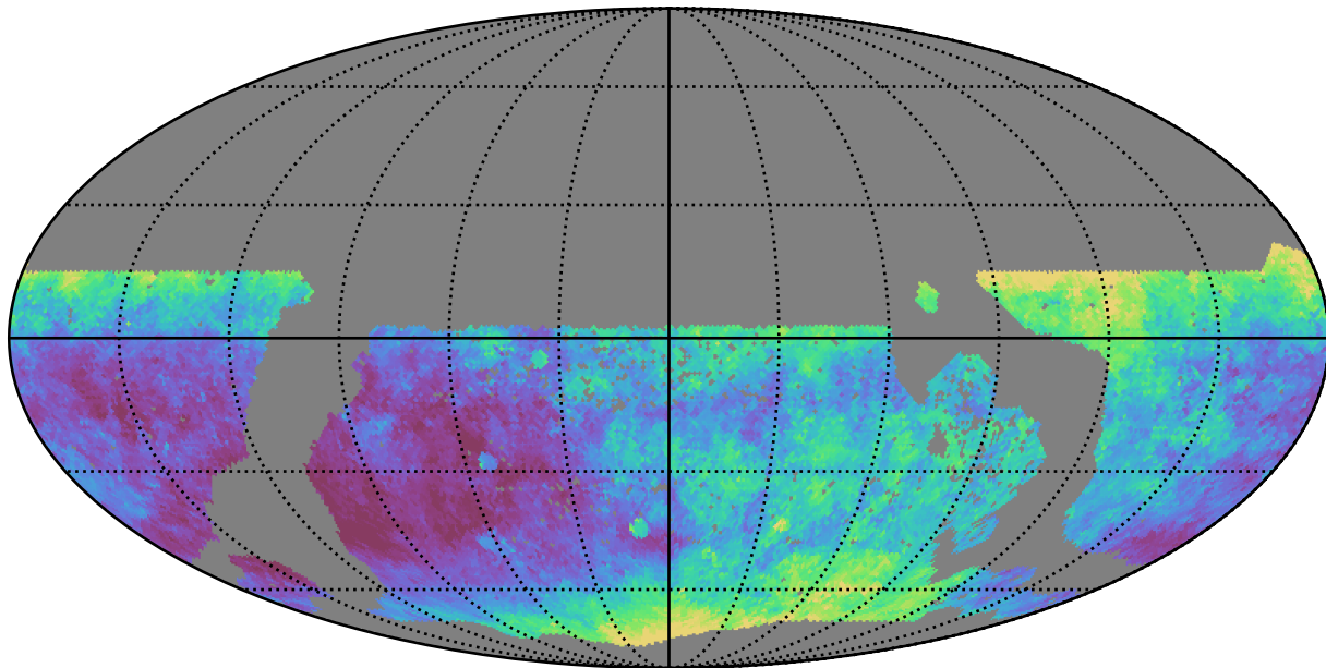
too_elab_r64_d2_griz_v3.4_10yrs WFD z band: Median seeingEff
