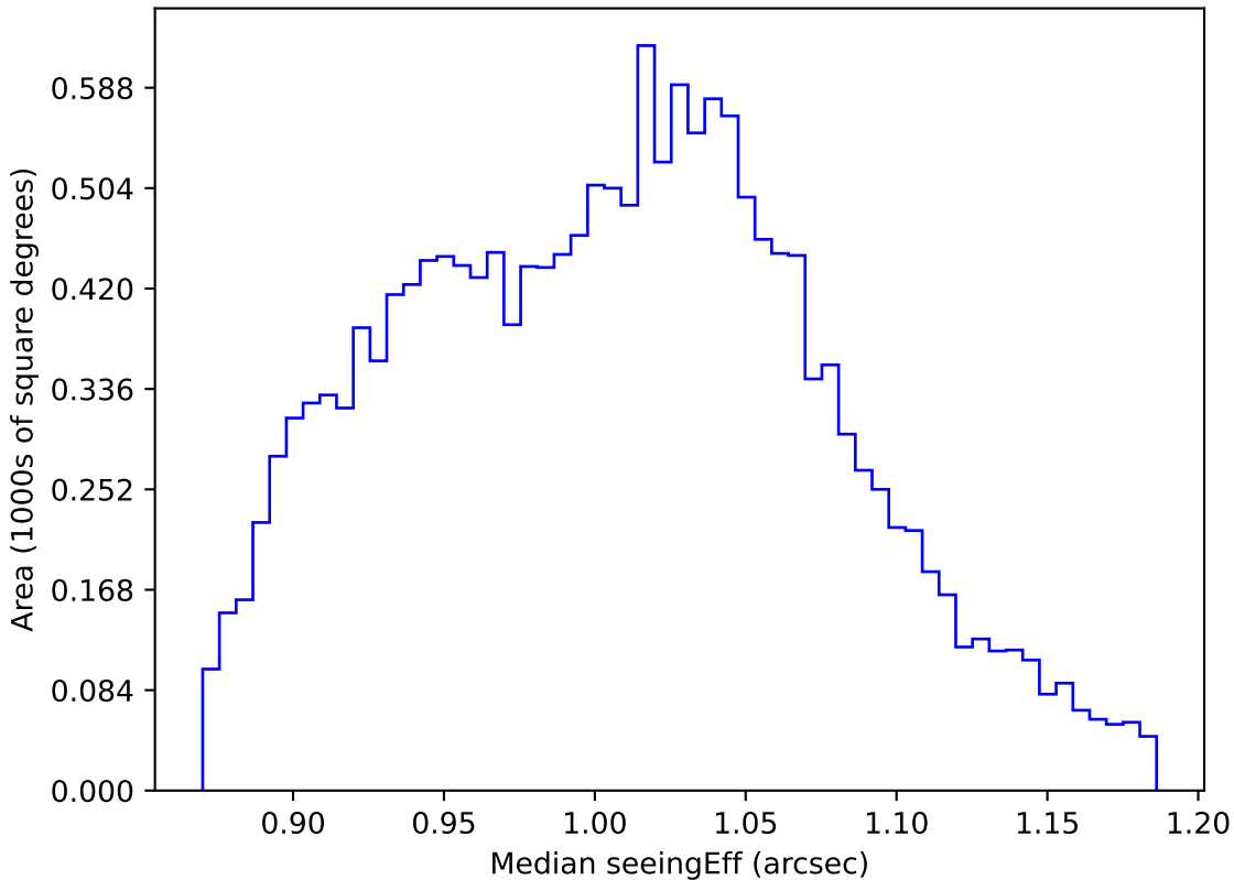
too_elab_r64_d2_griz_v3.4_10yrs WFD z band: Median seeingEff
