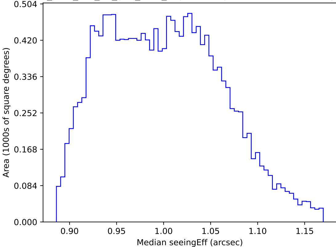
too_elab_r64_d2_griz_v3.4_10yrs WFD y band: Median seeingEff
