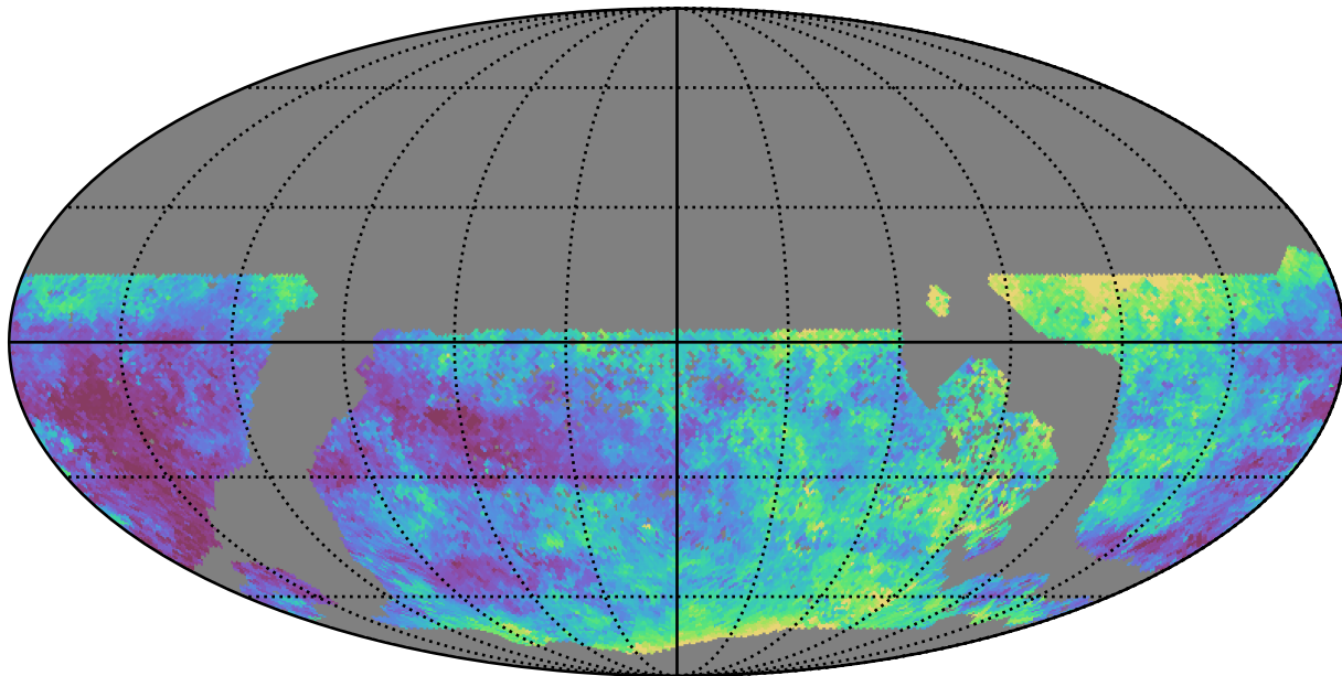
too_elab_r64_d2_griz_v3.4_10yrs WFD u band: Median seeingEff
