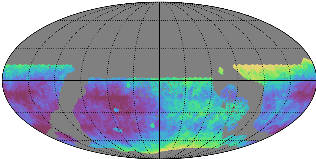
too_elab_r64_d2_griz_v3.4_10yrs WFD r band: Median seeingEff
