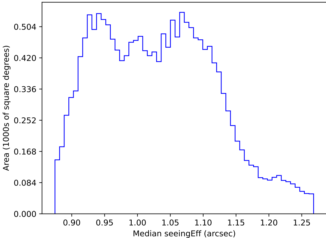
too_elab_r64_d2_griz_v3.4_10yrs WFD r band: Median seeingEff
