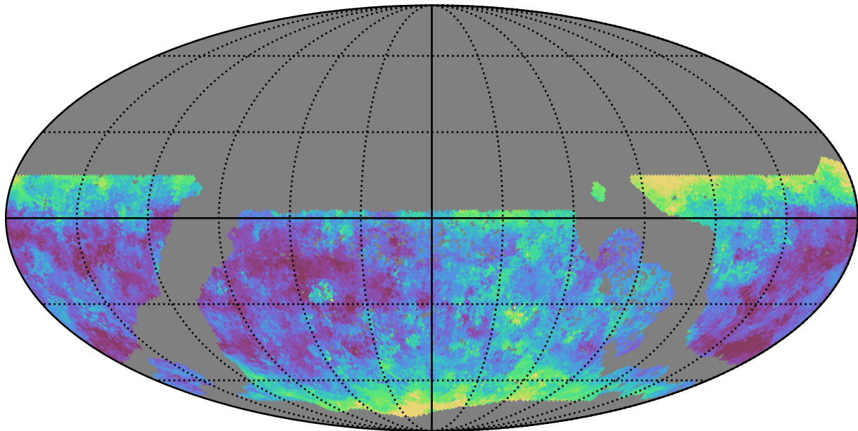
too_elab_r64_d2_griz_v3.4_10yrs WFD g band: Median seeingEff
