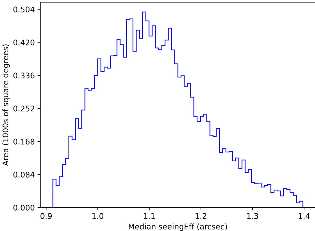
too_elab_r64_d2_griz_v3.4_10yrs WFD g band: Median seeingEff
