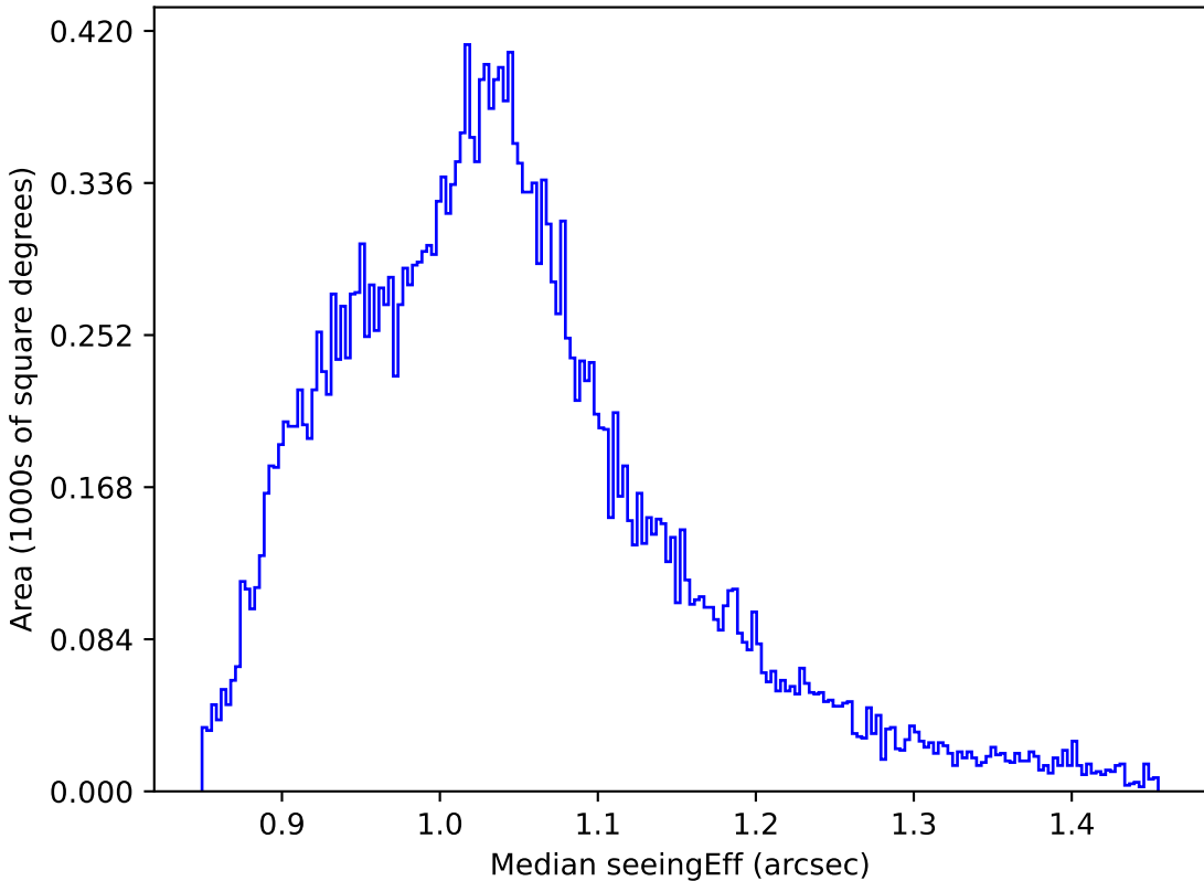
too_elab_r64_d2_griz_v3.4_10yrs All sky z band: Median seeingEff
