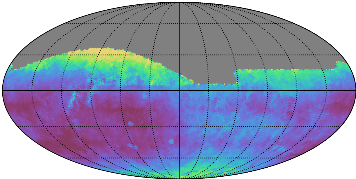
too_elab_r64_d2_griz_v3.4_10yrs All sky r band: Median seeingEff
