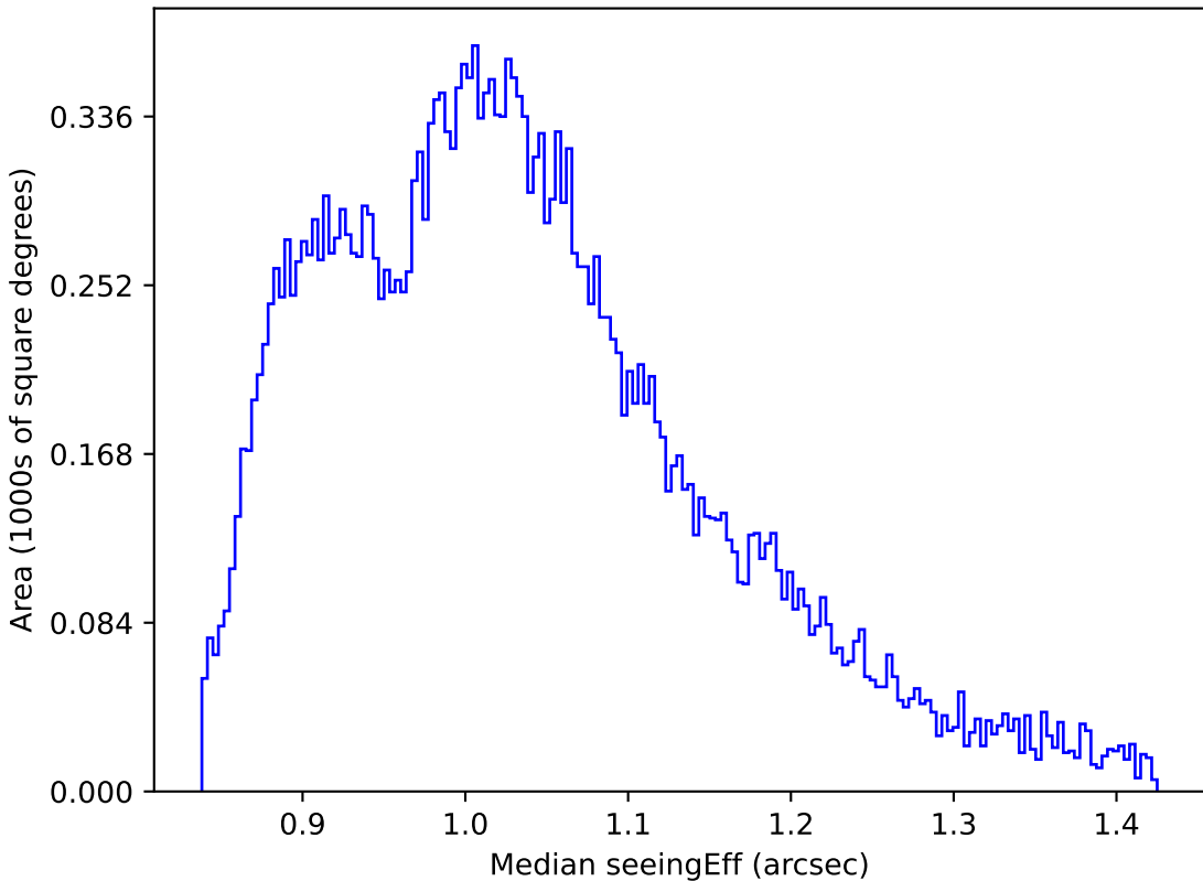
too_elab_r64_d2_griz_v3.4_10yrs All sky i band: Median seeingEff
