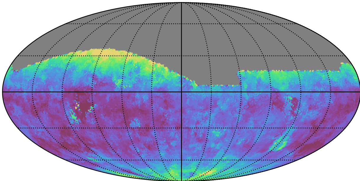
too_elab_r64_d2_griz_v3.4_10yrs All sky g band: Median seeingEff
