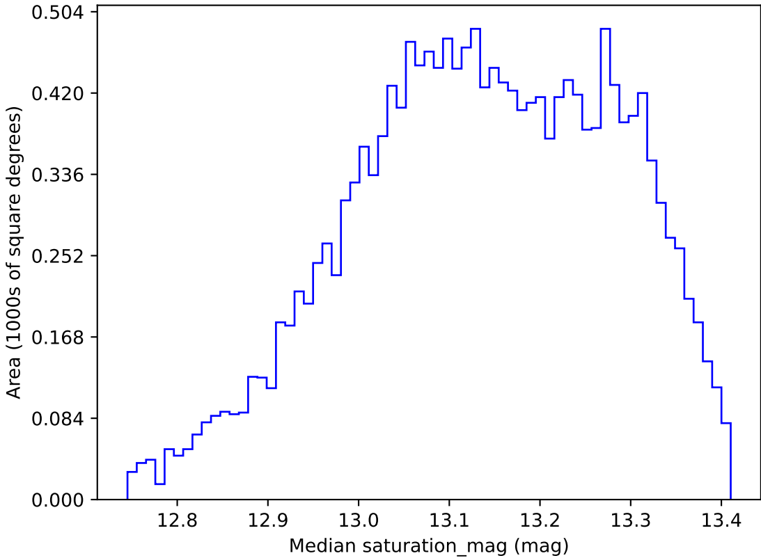
too_elab_r64_d2_griz_v3.4_10yrs WFD y band: Median saturation_mag
