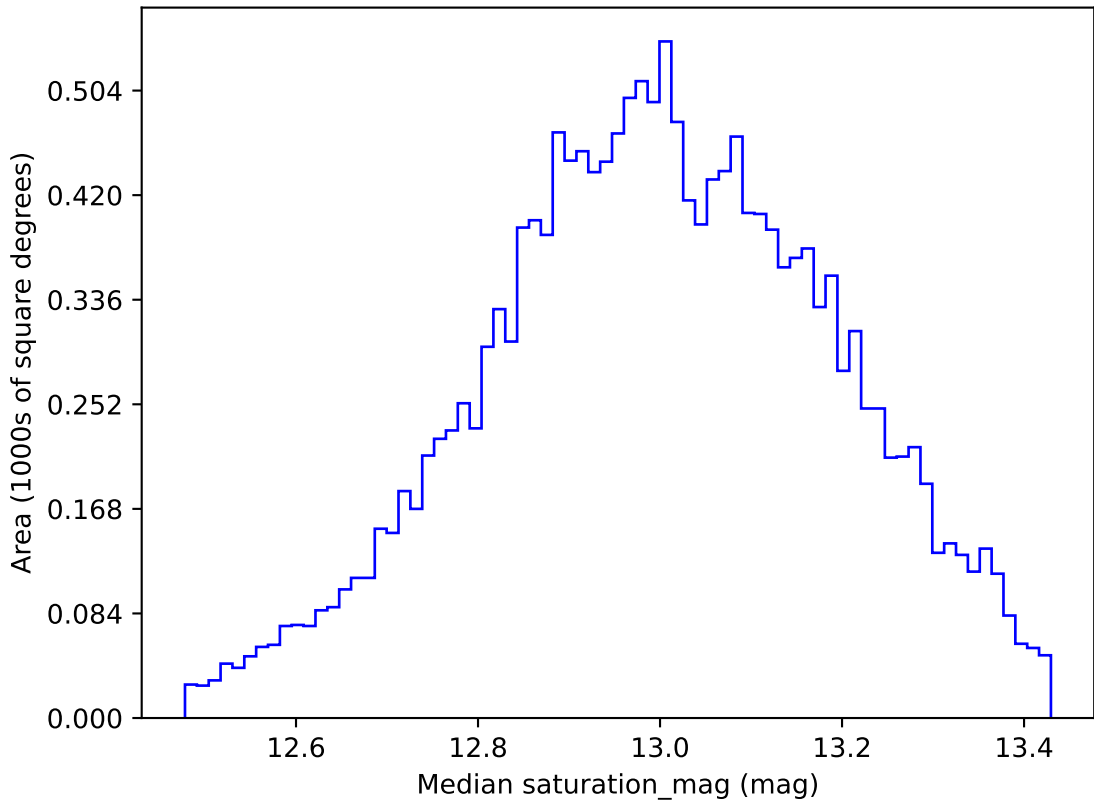
too_elab_r64_d2_griz_v3.4_10yrs WFD u band: Median saturation_mag
