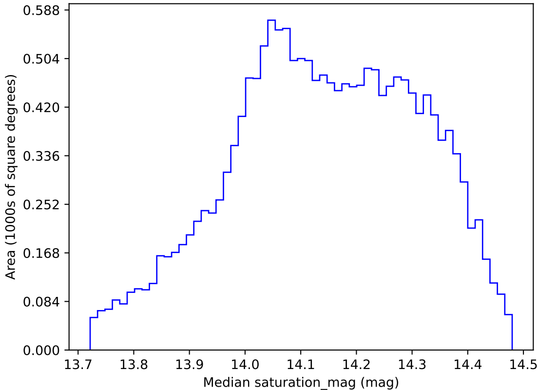
too_elab_r64_d2_griz_v3.4_10yrs WFD all bands: Median saturation_mag
