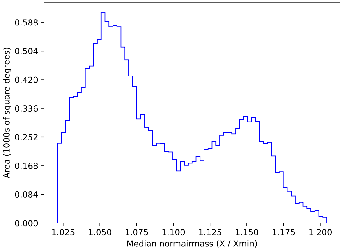
too_elab_r64_d2_griz_v3.4_10yrs WFD z band: Median normairmass
