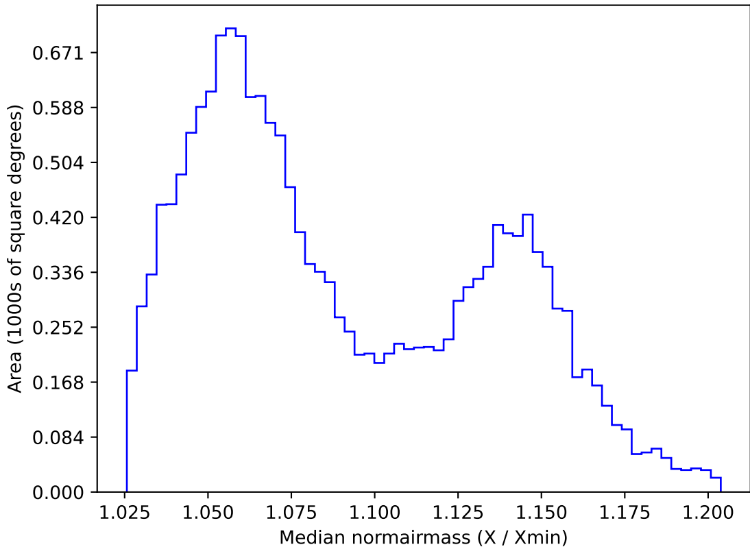
too_elab_r64_d2_griz_v3.4_10yrs WFD y band: Median normairmass
