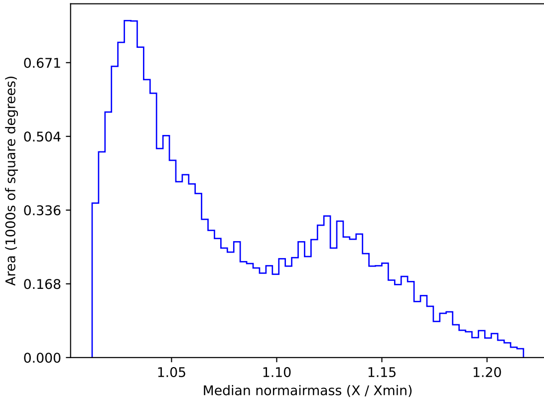
too_elab_r64_d2_griz_v3.4_10yrs WFD u band: Median normairmass
