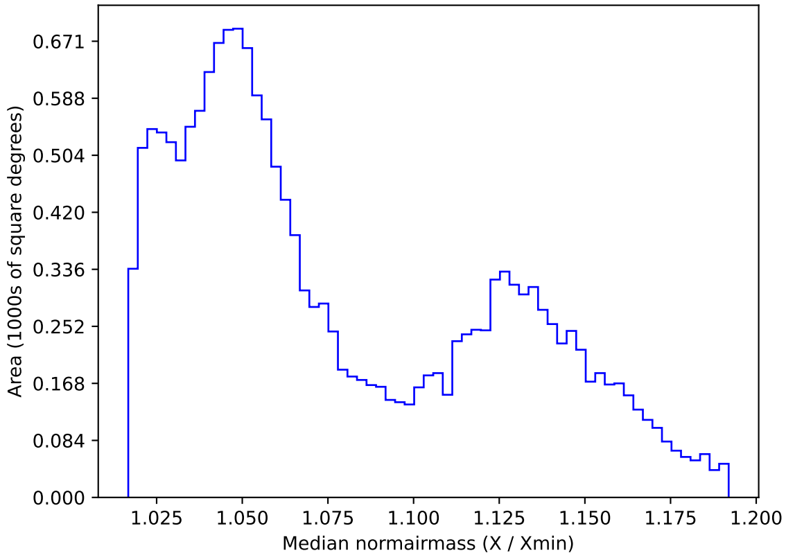
too_elab_r64_d2_griz_v3.4_10yrs WFD r band: Median normairmass
