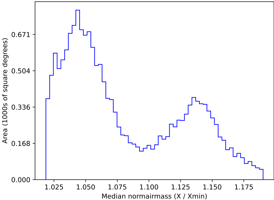
too_elab_r64_d2_griz_v3.4_10yrs WFD i band: Median normairmass
