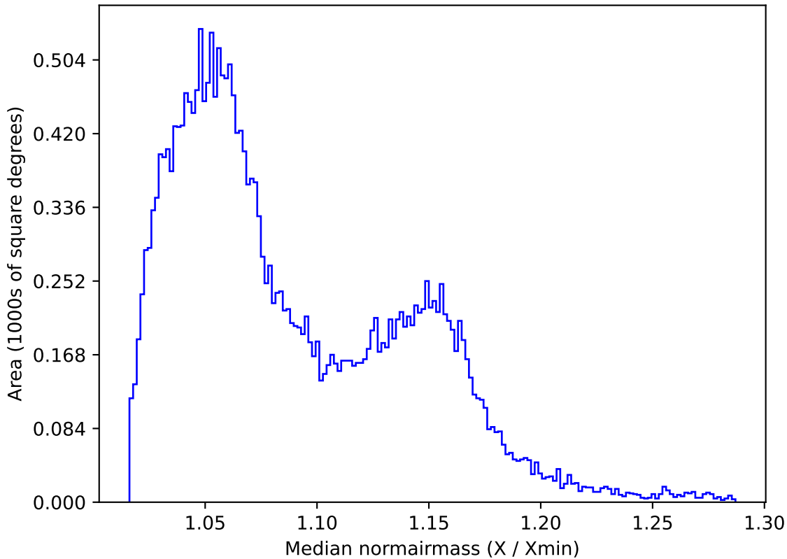
too_elab_r64_d2_griz_v3.4_10yrs All sky z band: Median normairmass
