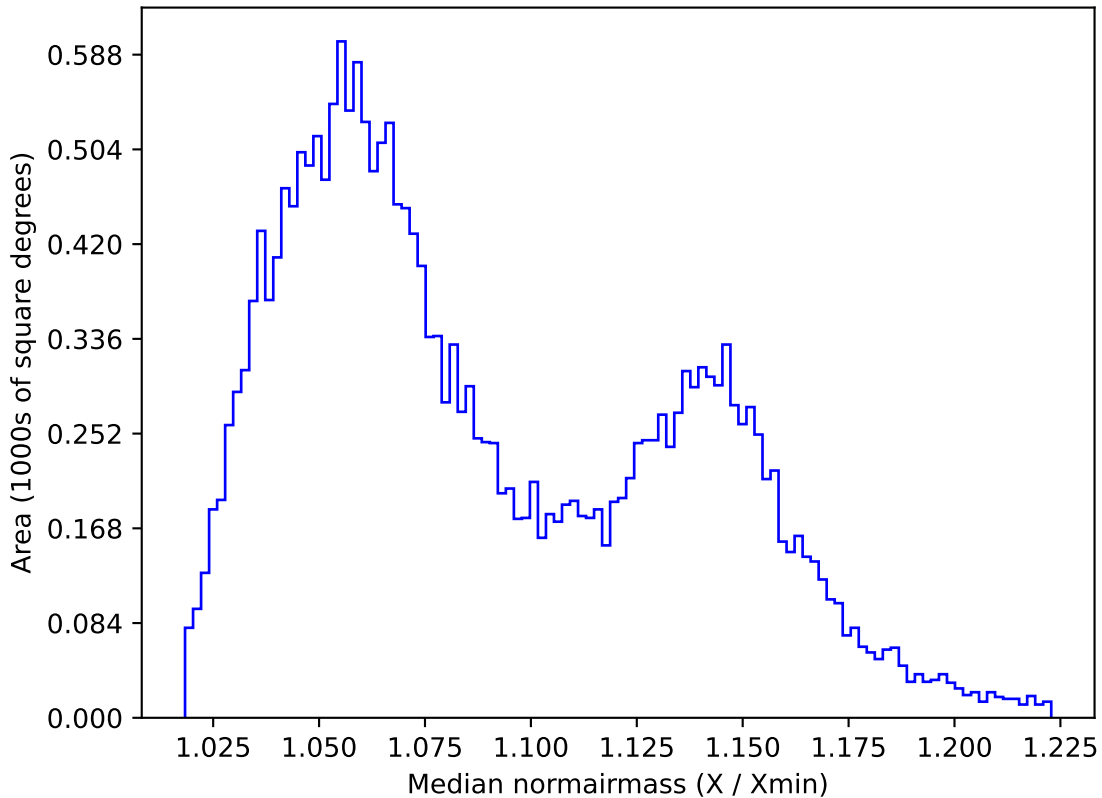
too_elab_r64_d2_griz_v3.4_10yrs All sky y band: Median normairmass
