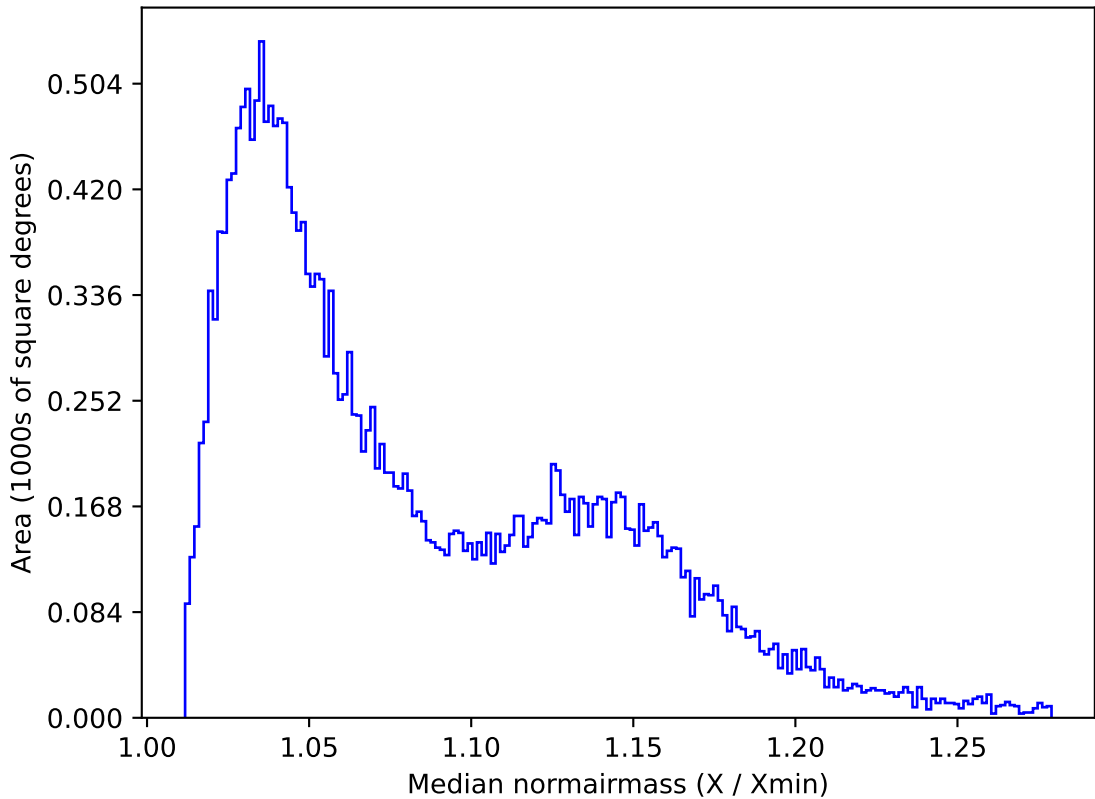
too_elab_r64_d2_griz_v3.4_10yrs All sky g band: Median normairmass
