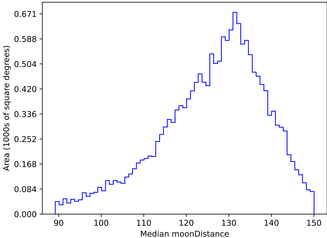
too_elab_r64_d2_griz_v3.4_10yrs WFD u band: Median moonDistance
