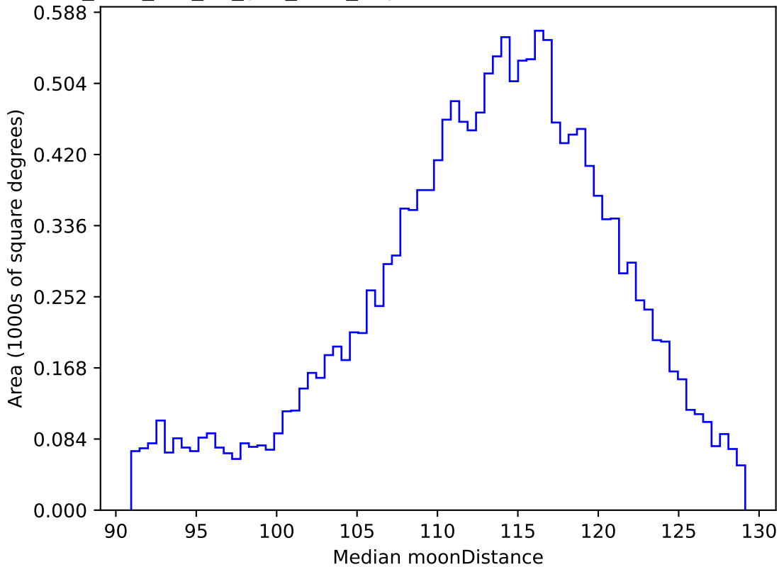
too_elab_r64_d2_griz_v3.4_10yrs WFD r band: Median moonDistance
