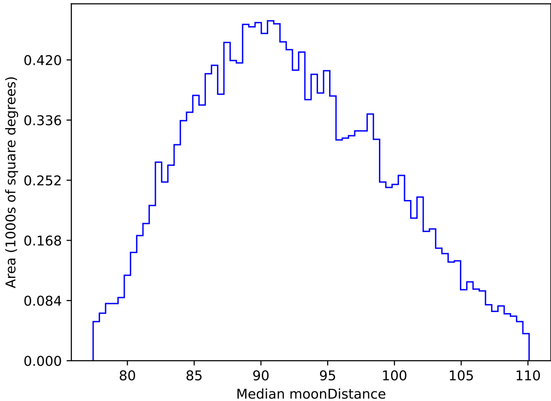
too_elab_r64_d2_griz_v3.4_10yrs WFD i band: Median moonDistance
