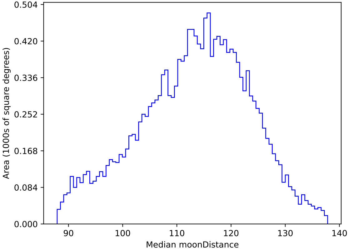
too_elab_r64_d2_griz_v3.4_10yrs WFD g band: Median moonDistance
