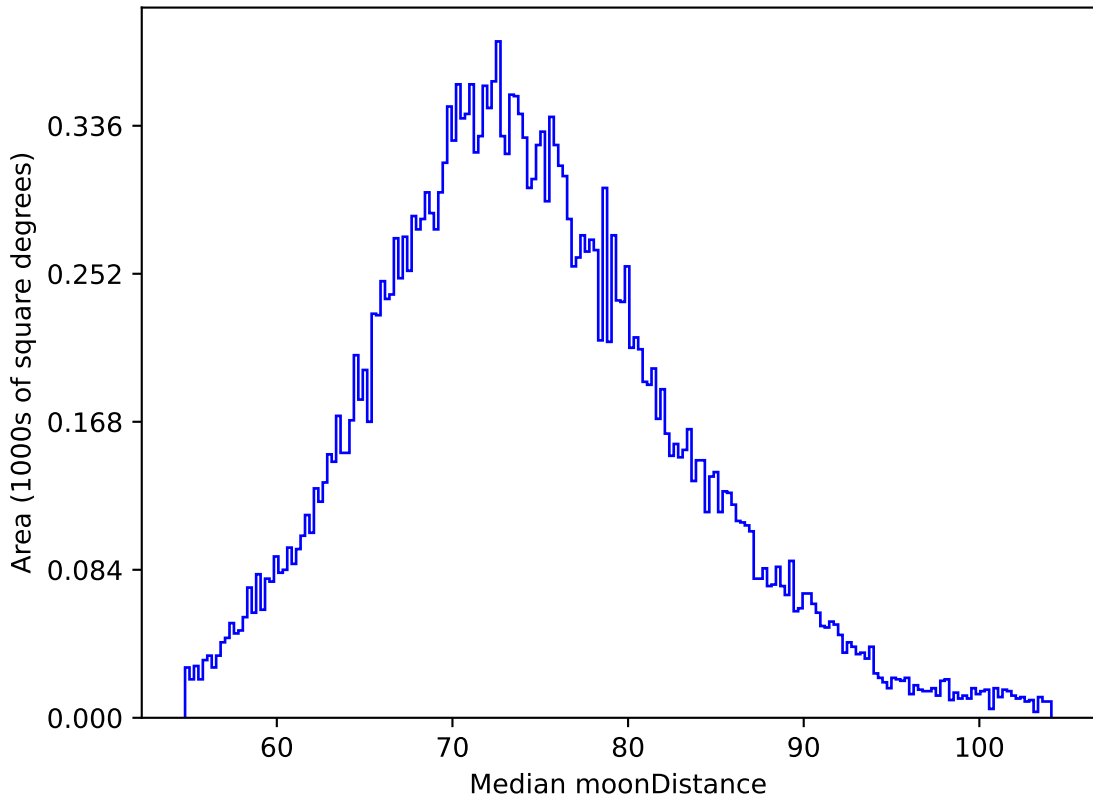
too_elab_r64_d2_griz_v3.4_10yrs All sky z band: Median moonDistance
