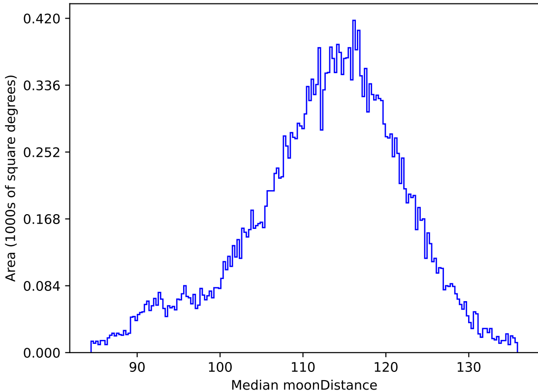
too_elab_r64_d2_griz_v3.4_10yrs All sky r band: Median moonDistance
