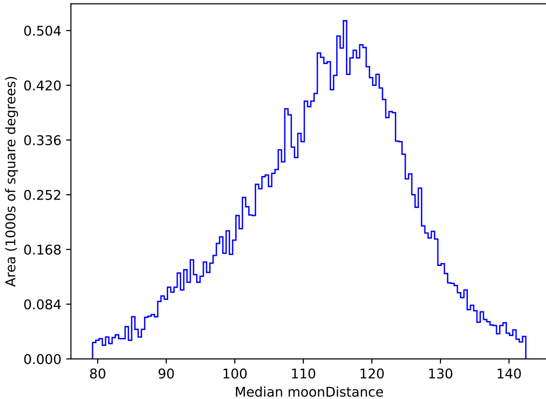
too_elab_r64_d2_griz_v3.4_10yrs All sky g band: Median moonDistance
