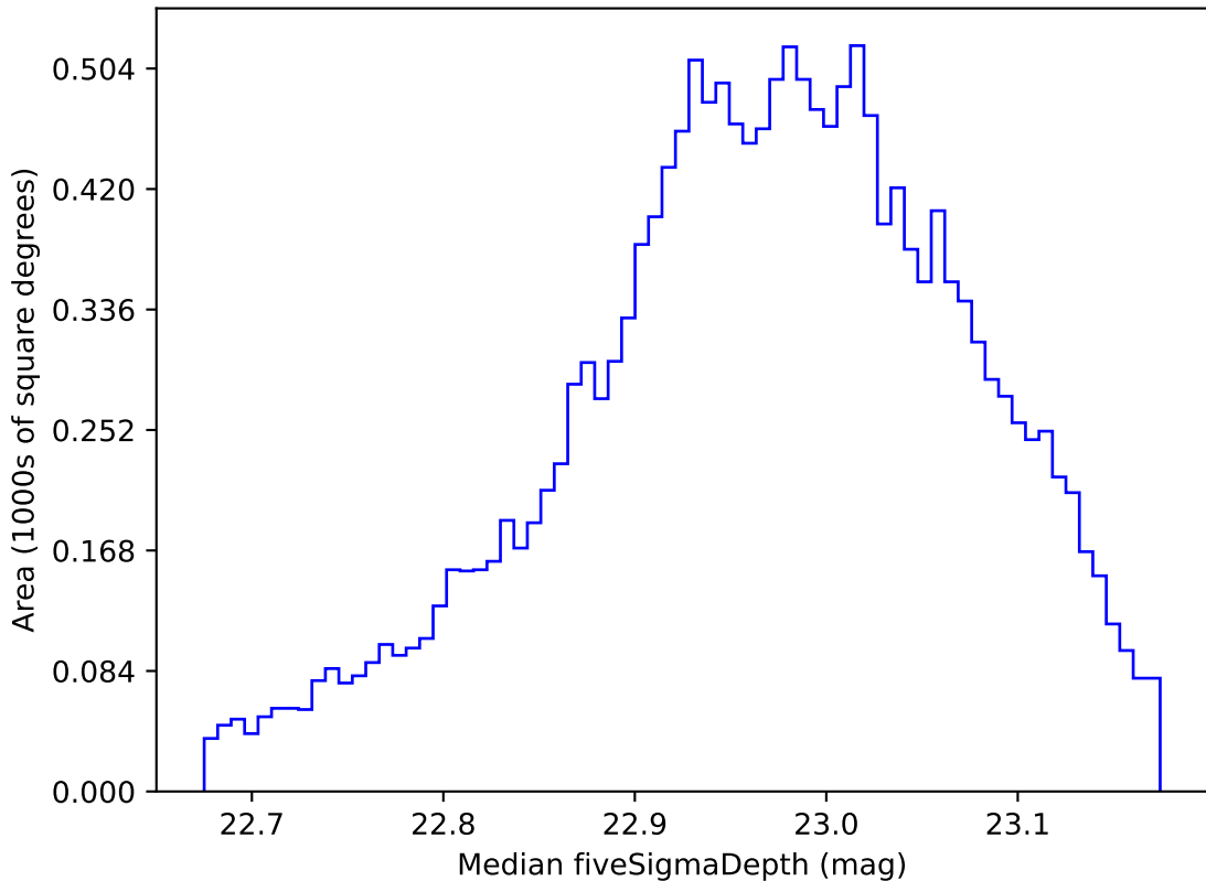
too_elab_r64_d2_griz_v3.4_10yrs WFD z band: Median fiveSigmaDepth
