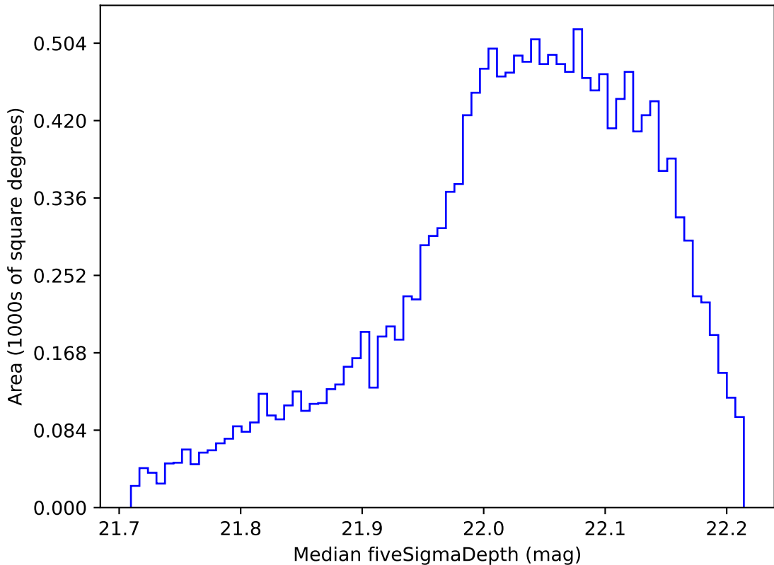
too_elab_r64_d2_griz_v3.4_10yrs WFD y band: Median fiveSigmaDepth
