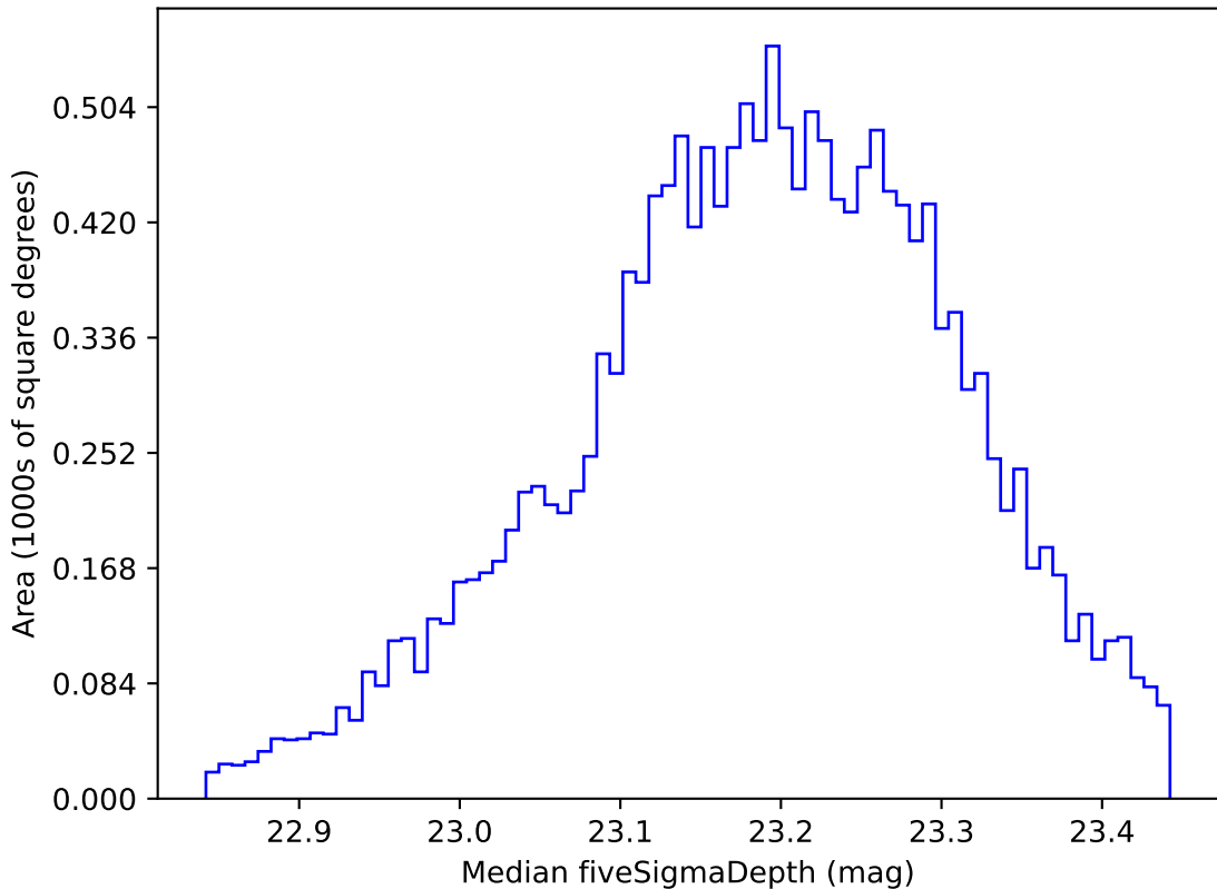
too_elab_r64_d2_griz_v3.4_10yrs WFD u band: Median fiveSigmaDepth
